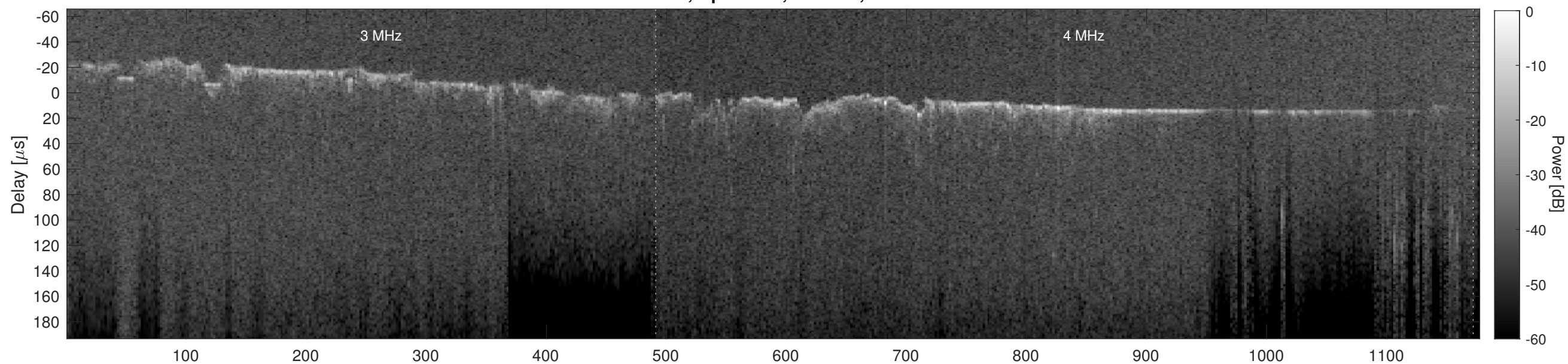
Orbit 12409, Cluttergram
