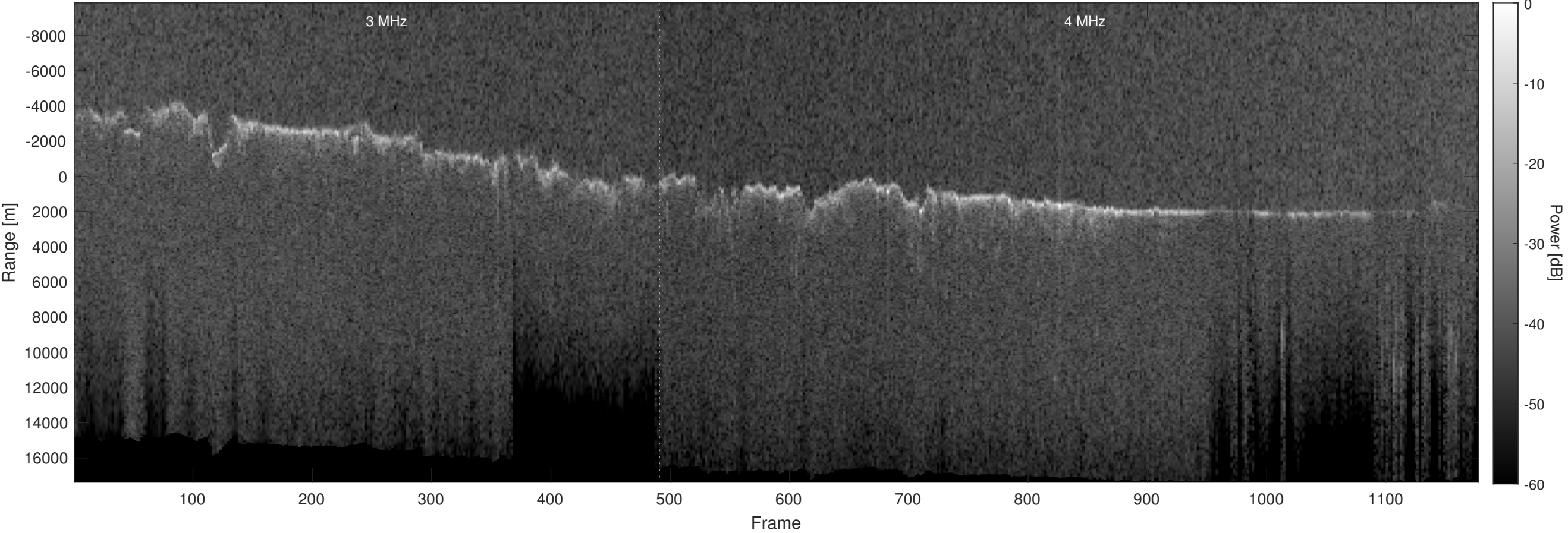
Orbit 12409, Optimized, Window, Depth-Corrected, Channel 2
