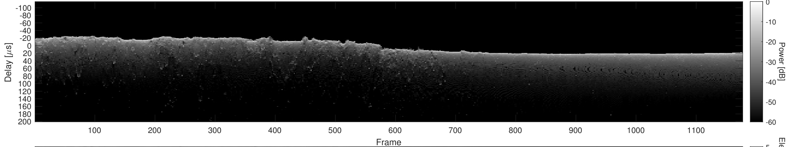
Orbit 12411, Cluttergram
