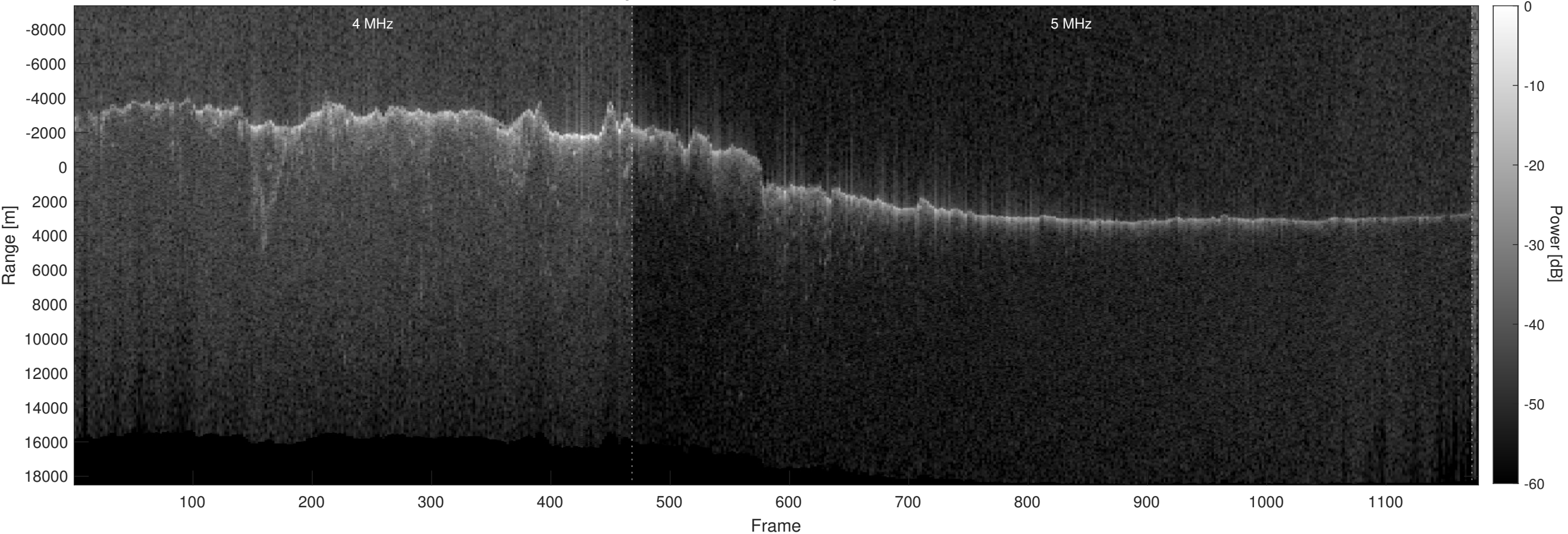
Orbit 12411, Optimized, No Window, Depth-Corrected, Channel 2
