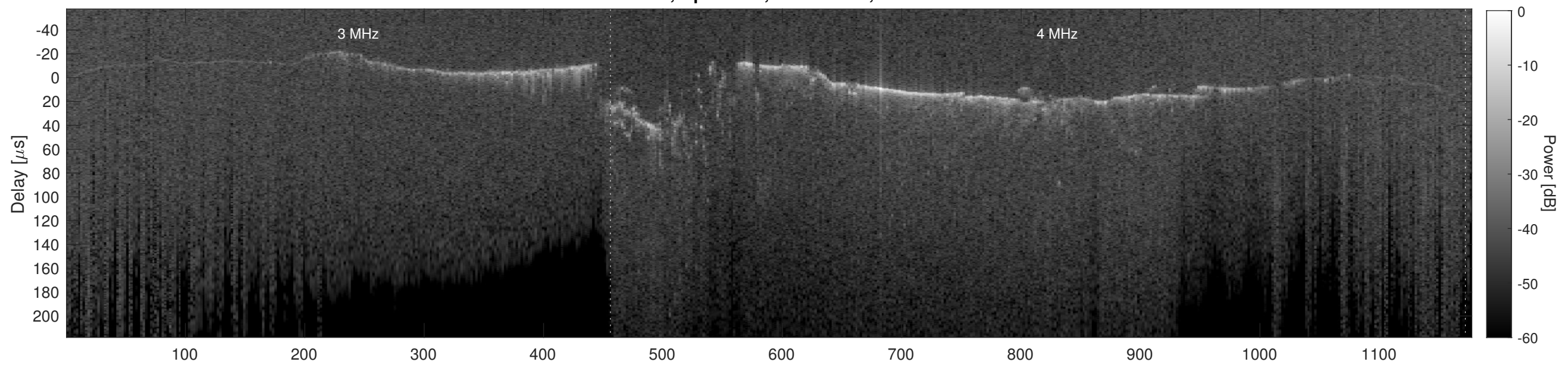
Orbit 12413, Cluttergram
