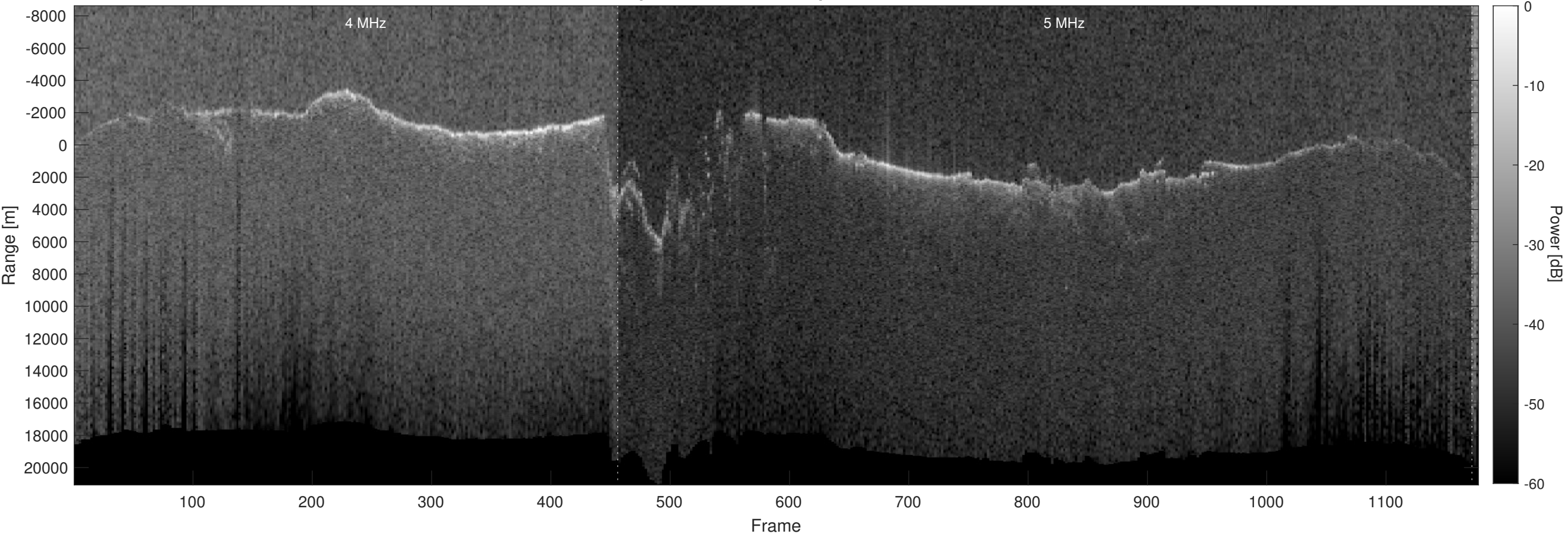
Orbit 12413, Optimized, Window, Depth-Corrected, Channel 2
