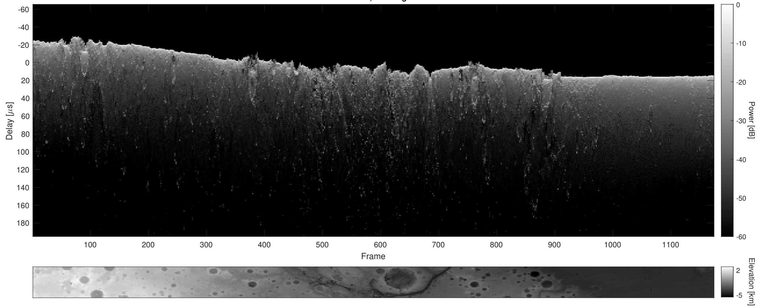
Orbit 12416, Cluttergram
