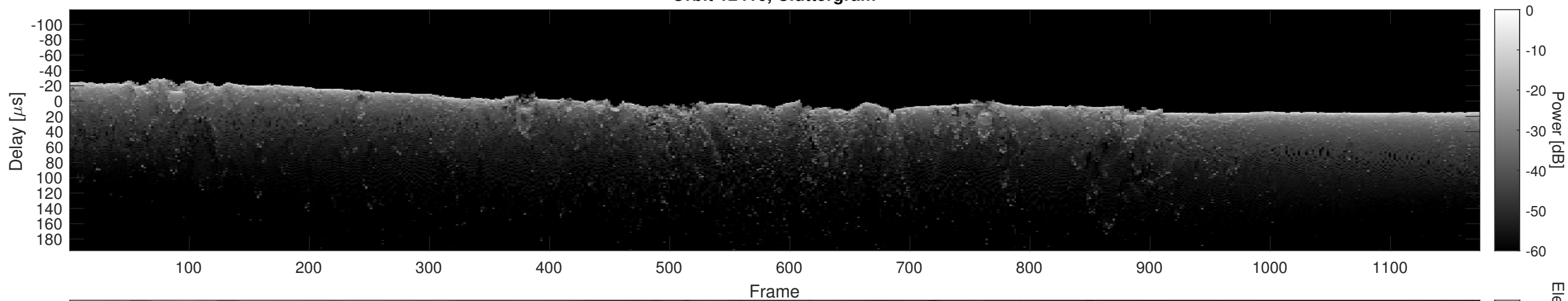
Orbit 12416, Cluttergram
