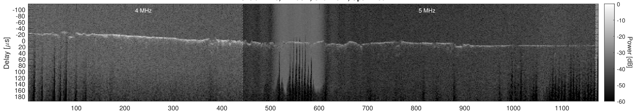
Orbit 12416, Cluttergram
