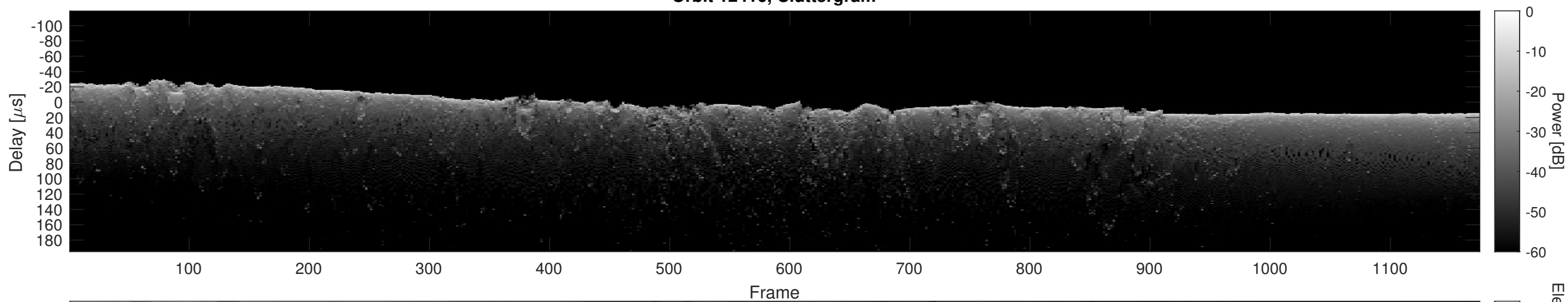
Orbit 12416, Cluttergram
