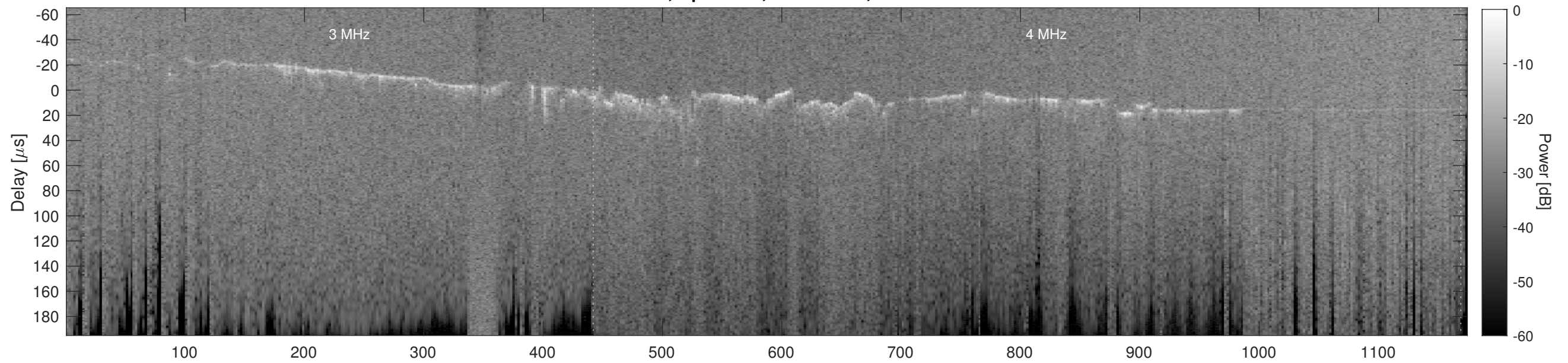
Orbit 12416, Cluttergram
