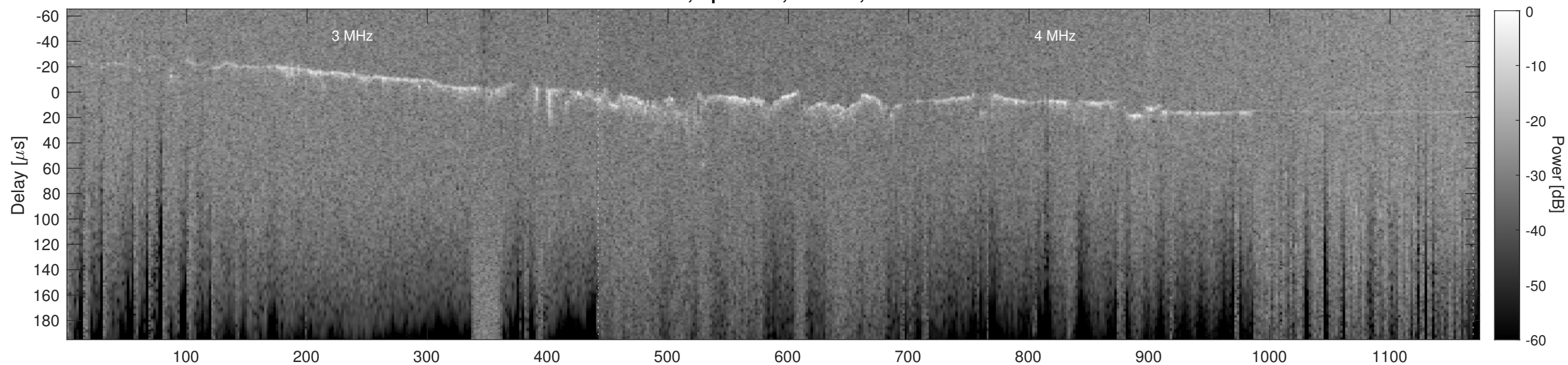
Orbit 12416, Cluttergram
