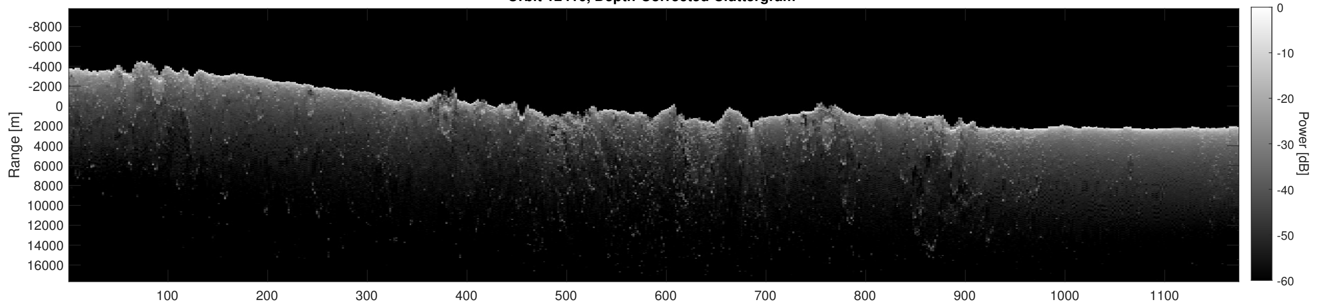
Orbit 12416, Depth-Corrected Cluttergram
