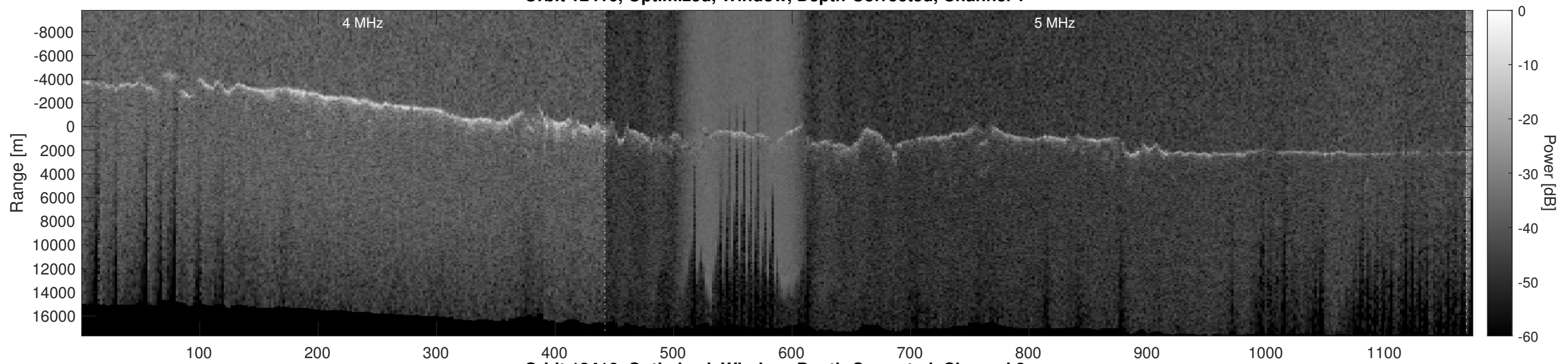
Orbit 12416, Optimized, Window, Depth-Corrected, Channel 2
