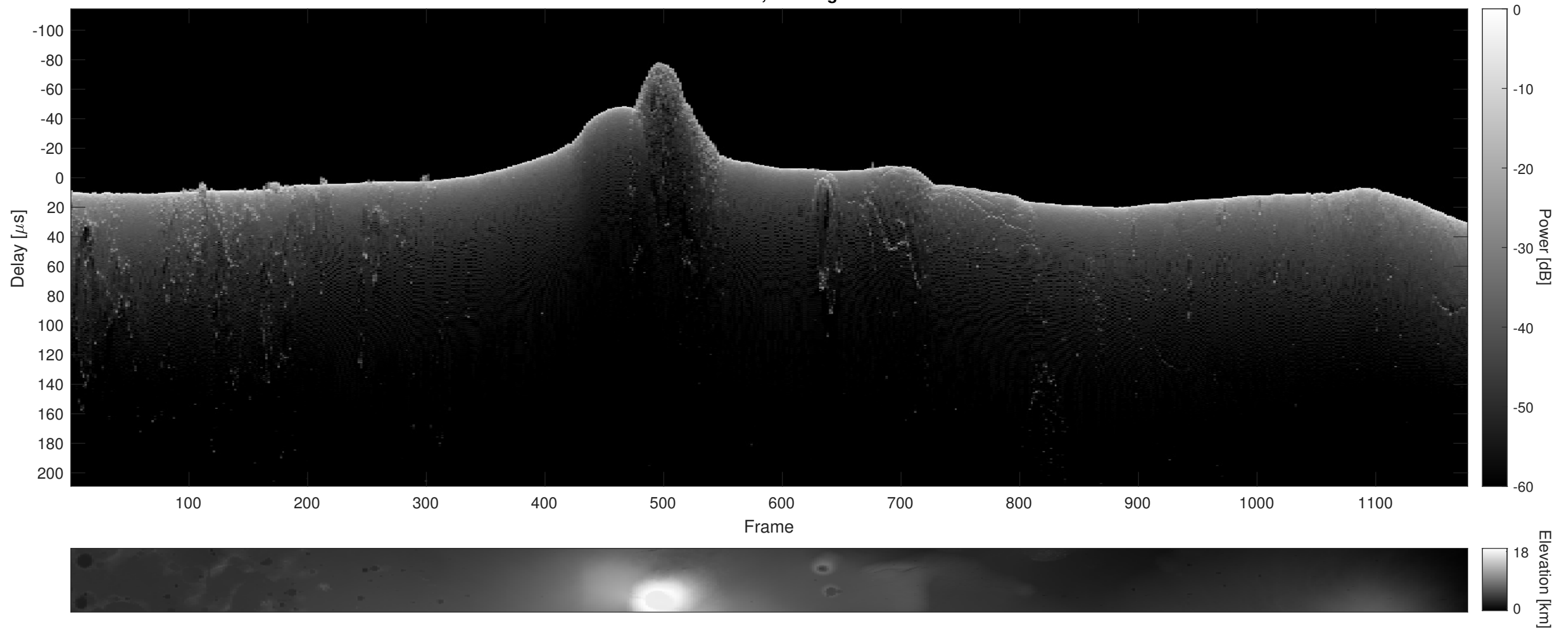
Orbit 12417, Cluttergram
