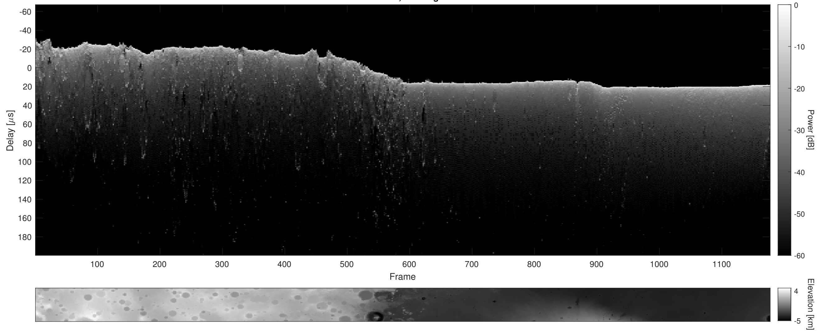
Orbit 12418, Cluttergram
