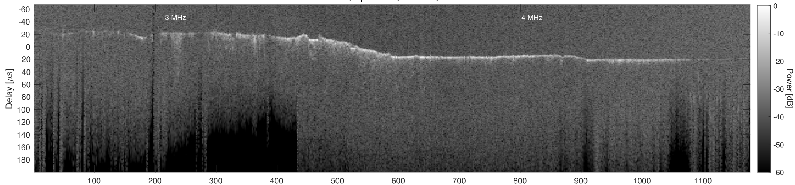
Orbit 12418, Cluttergram
