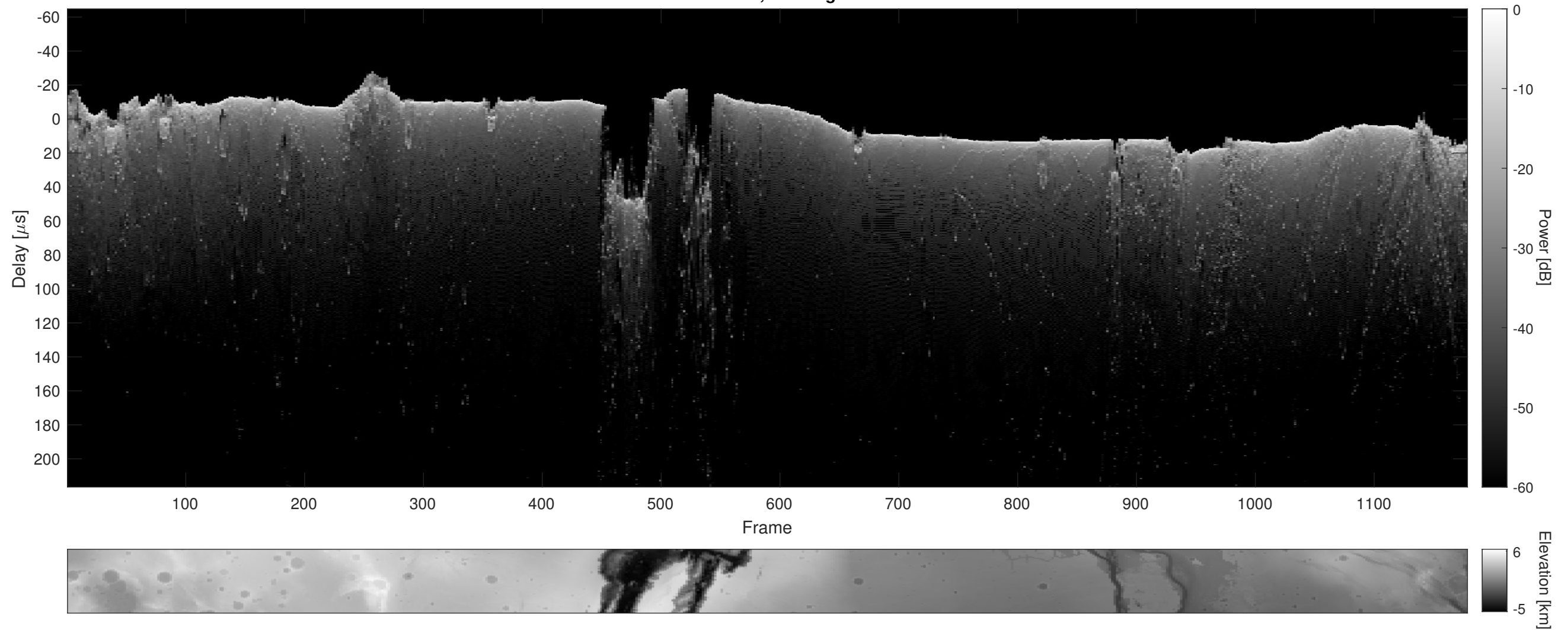
Orbit 12420, Cluttergram
