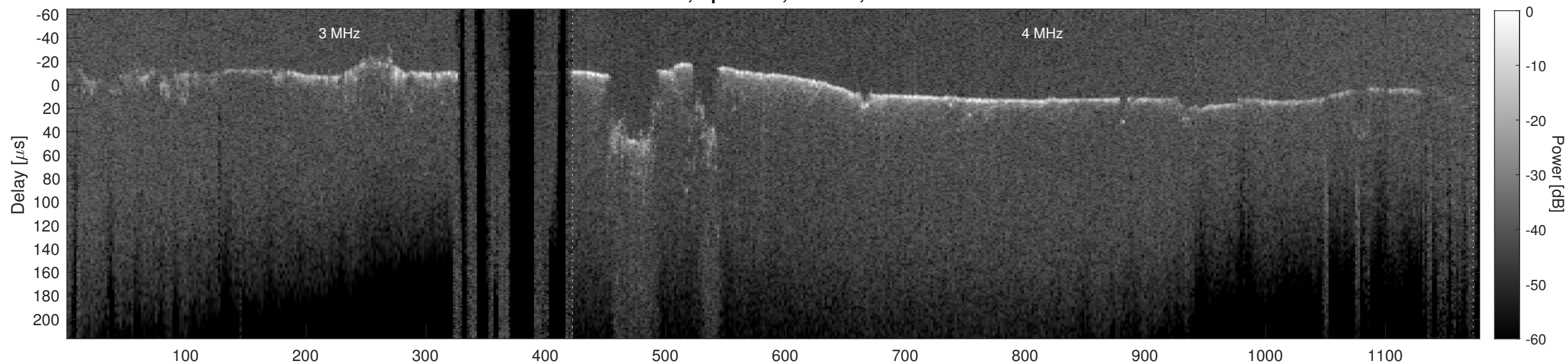
Orbit 12420, Cluttergram
