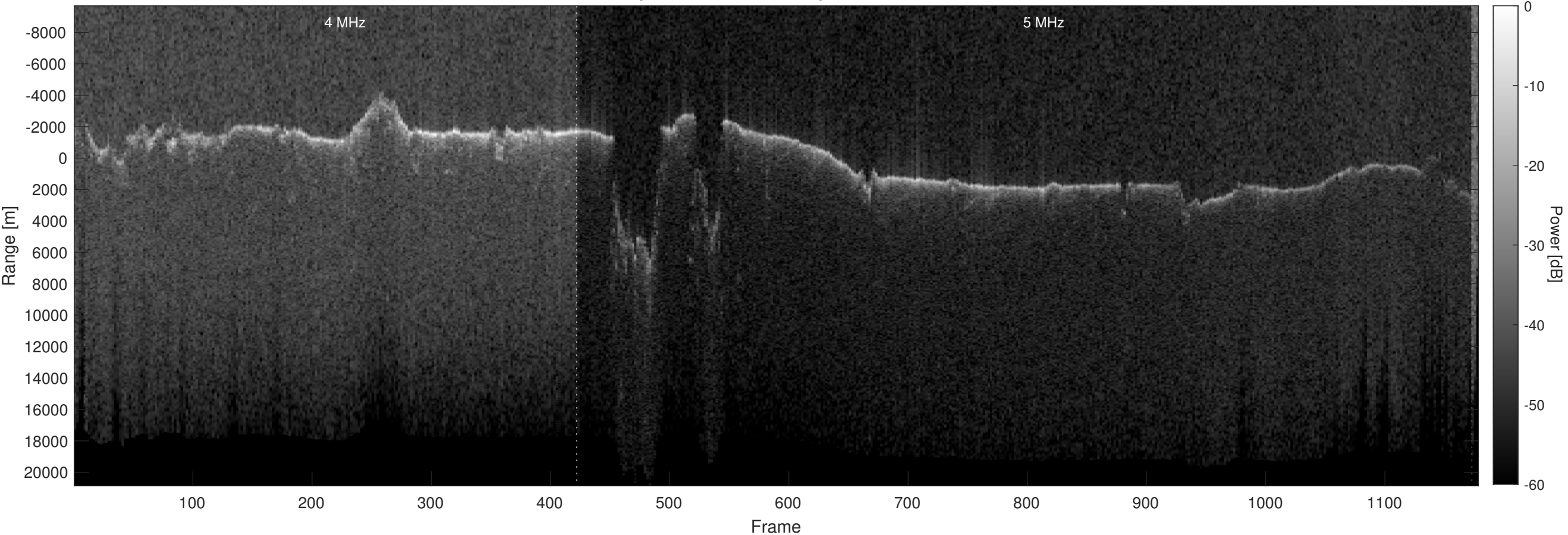
Orbit 12420, Optimized, Window, Depth-Corrected, Channel 2
