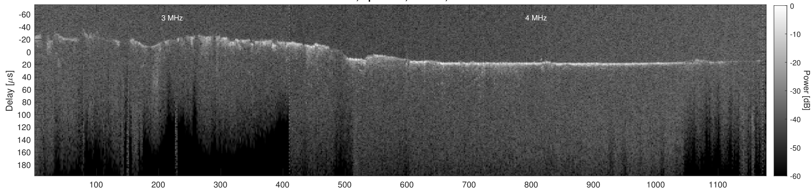
Orbit 12421, Cluttergram
