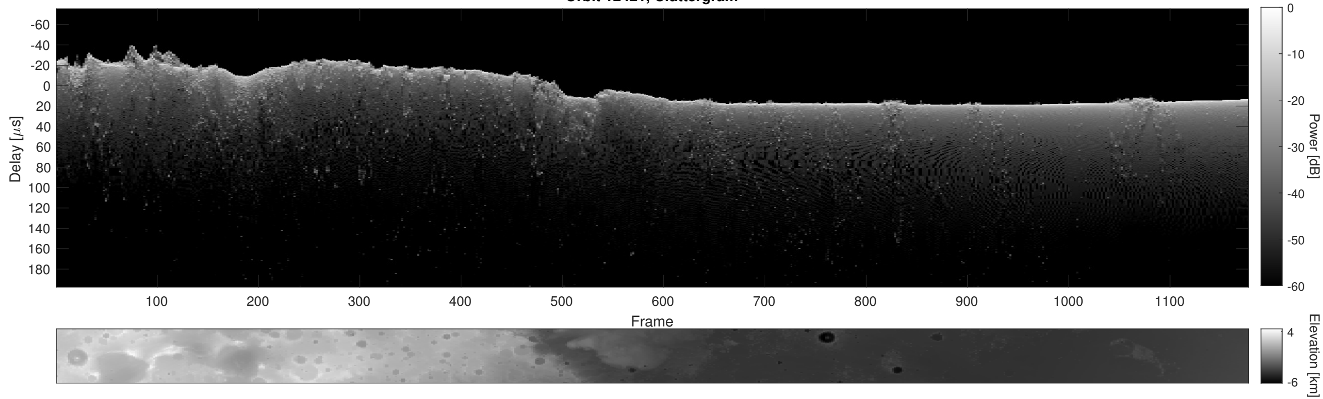
Orbit 12421, Cluttergram
