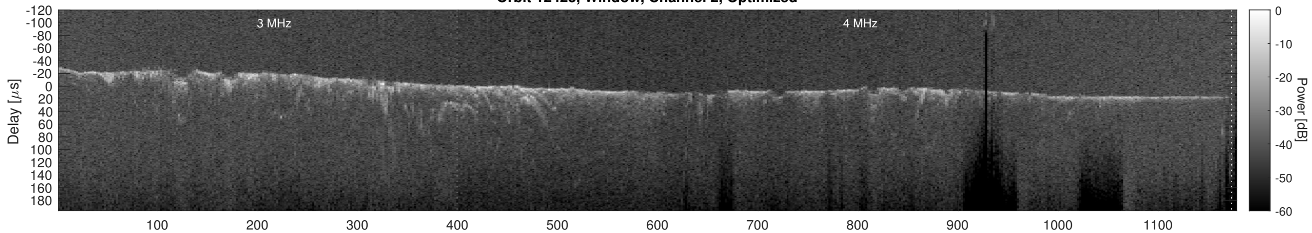
Orbit 12423, Cluttergram
