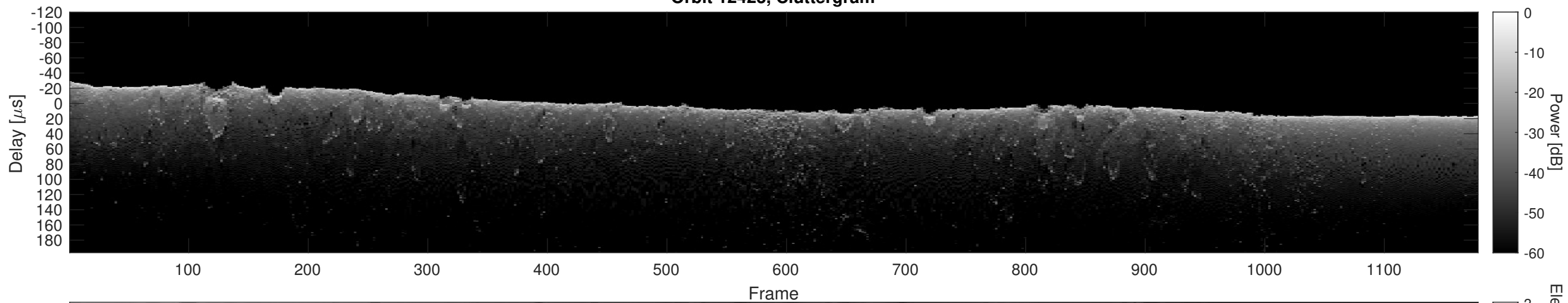
Orbit 12423, Cluttergram
