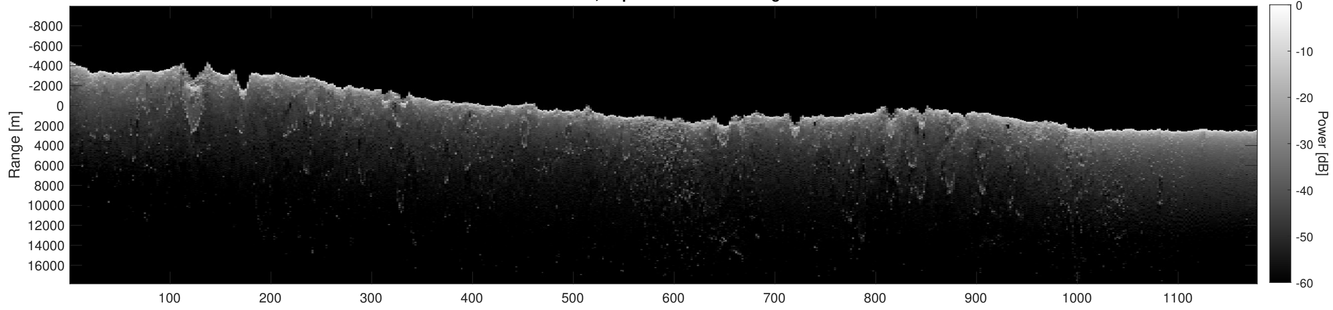
Orbit 12423, Depth-Corrected Cluttergram
