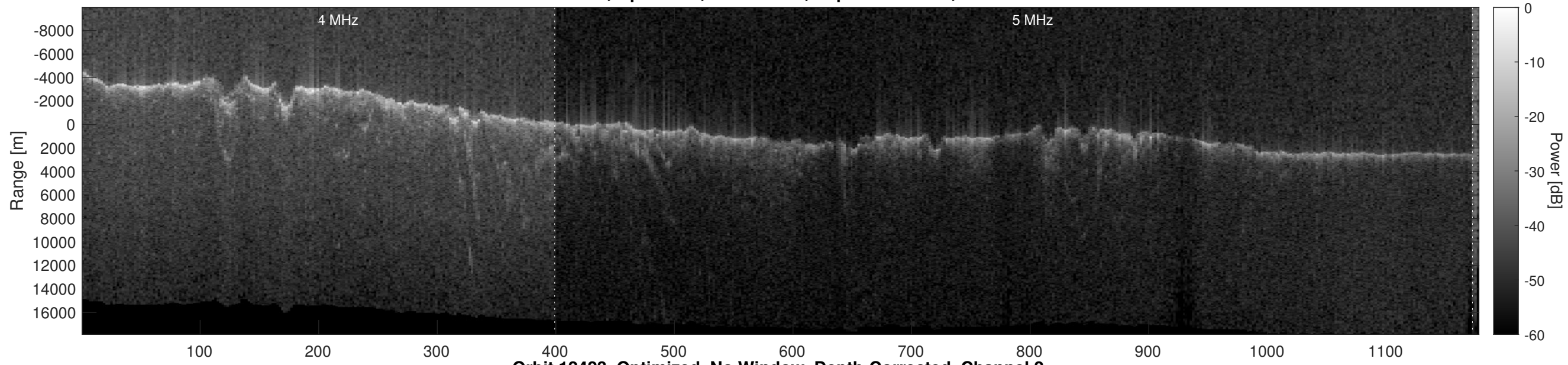
Orbit 12423, Optimized, No Window, Depth-Corrected, Channel 2
