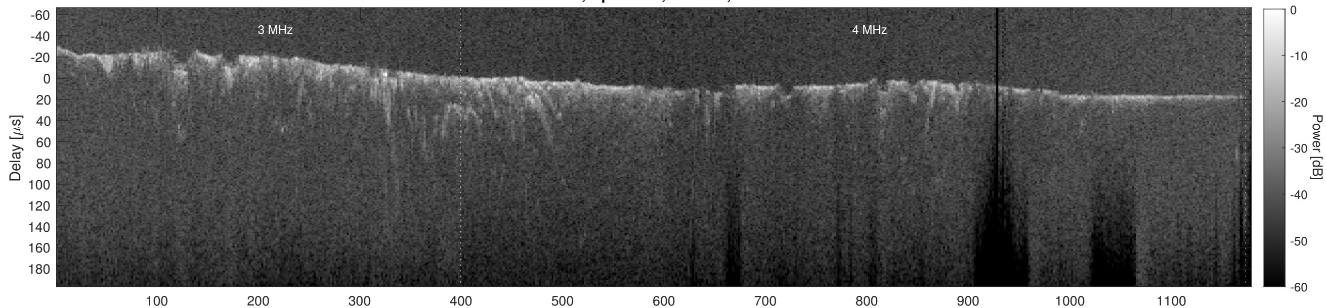
Orbit 12423, Cluttergram
