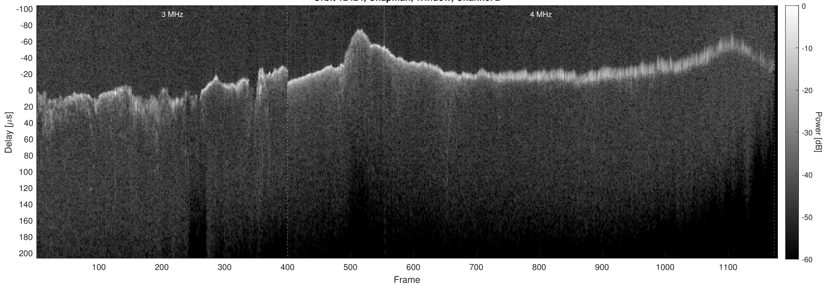
Orbit 12424, Chapman, Window, Channel 2
