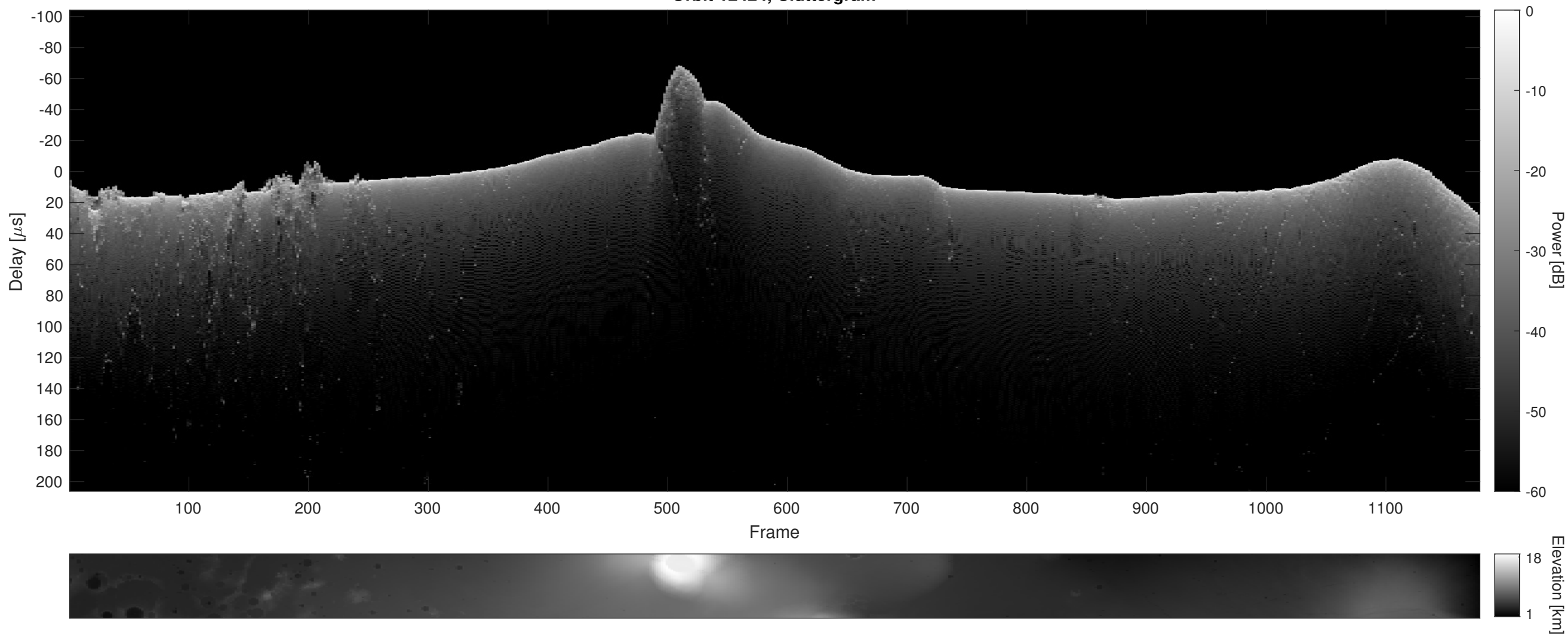
Orbit 12424, Cluttergram
