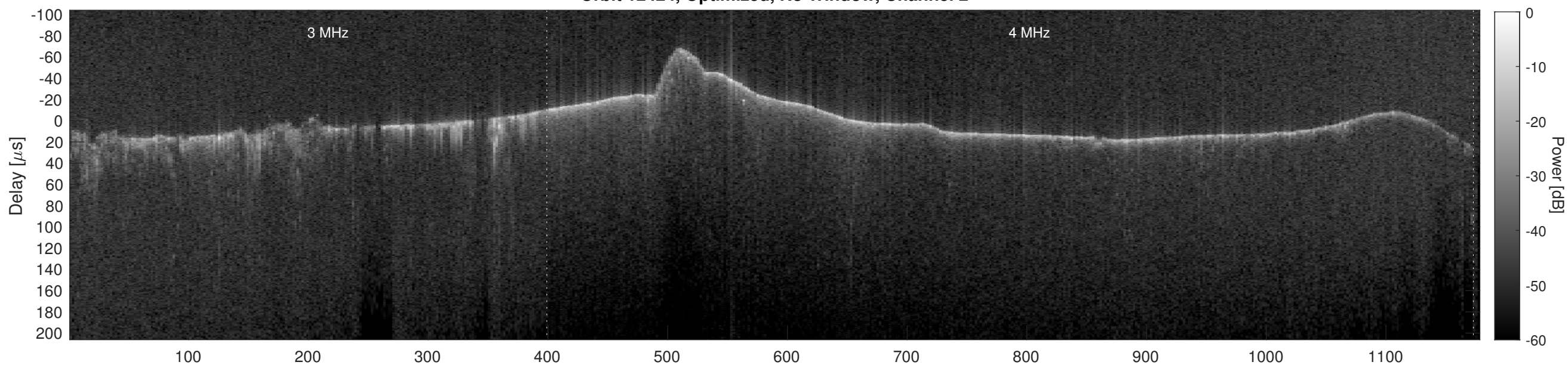
Orbit 12424, Cluttergram
