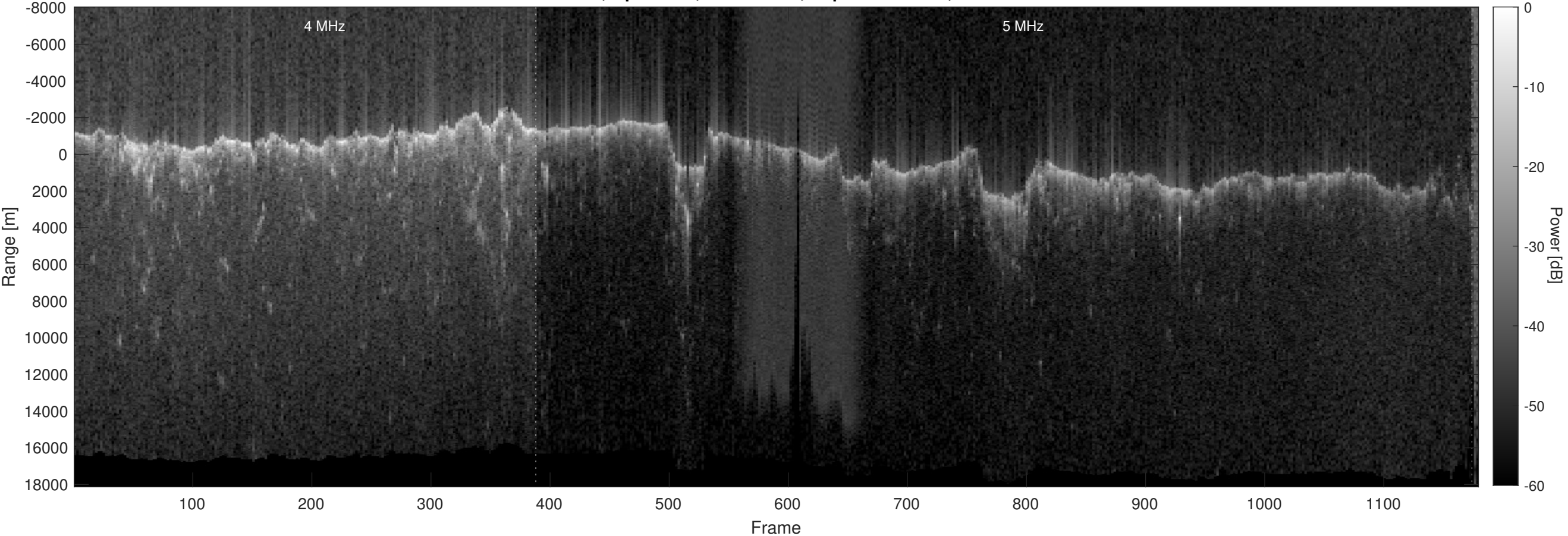
Orbit 12426, Optimized, No Window, Depth-Corrected, Channel 2
