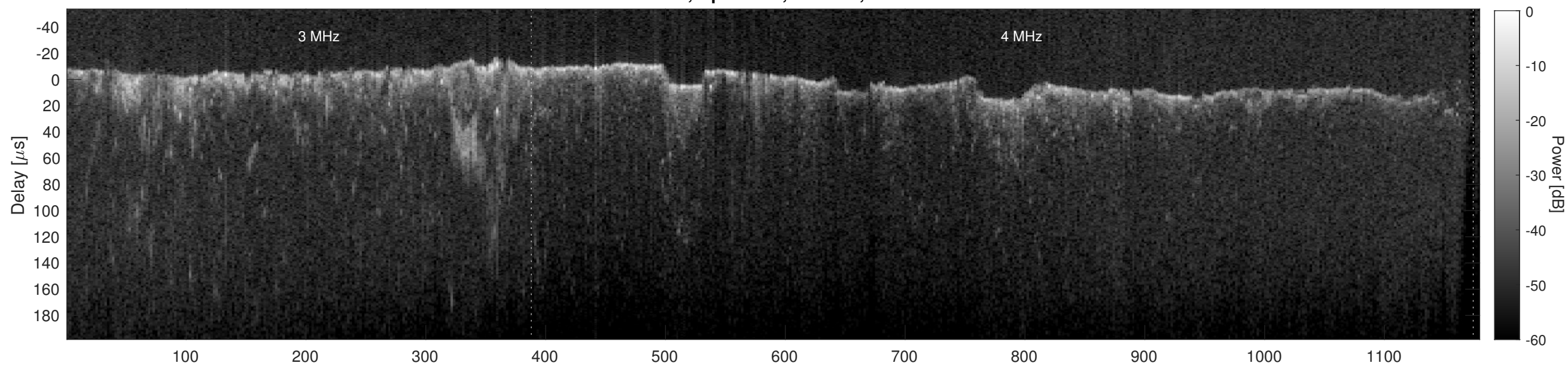
Orbit 12426, Cluttergram
