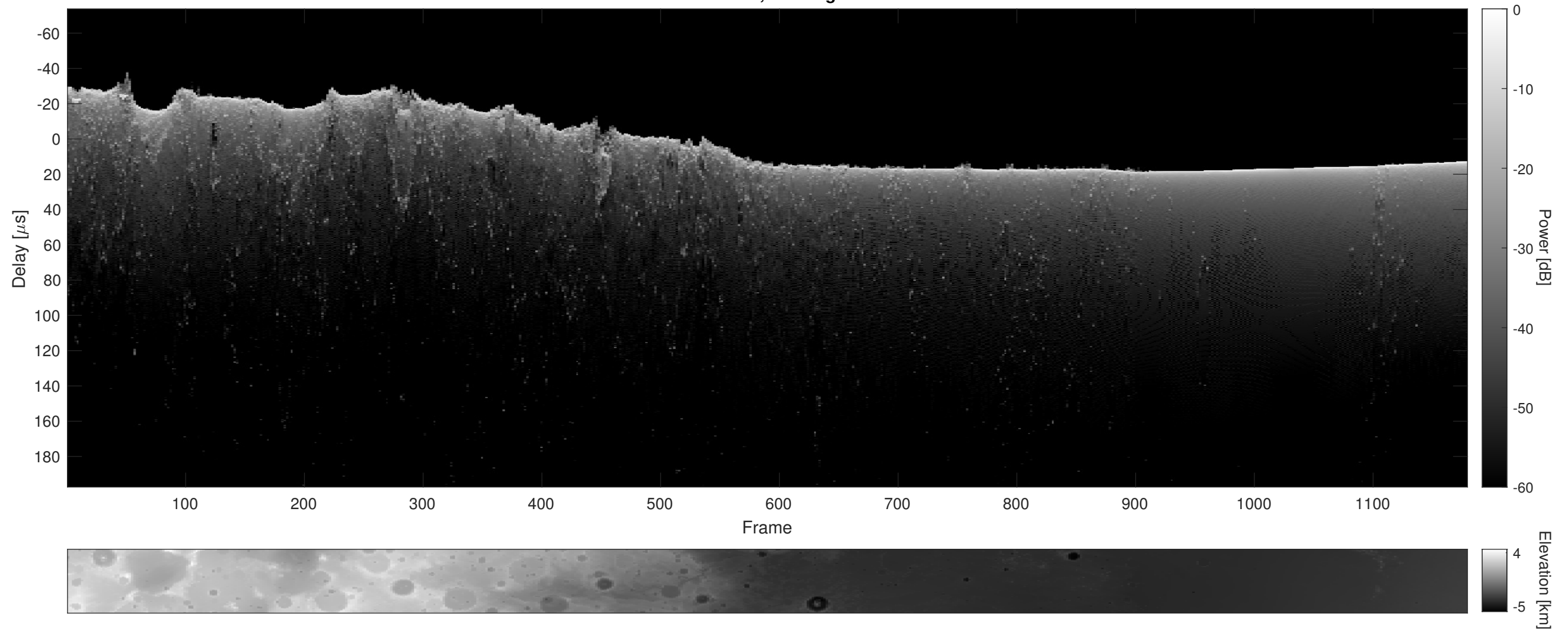
Orbit 12428, Cluttergram
