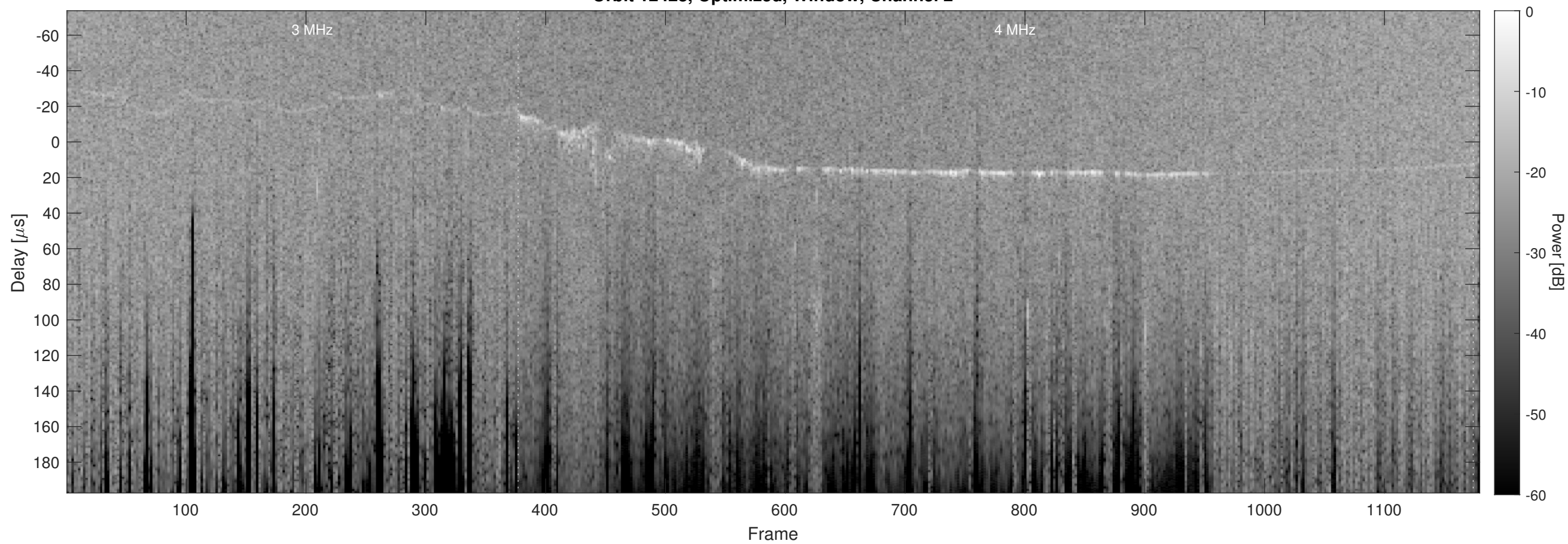
Orbit 12428, Optimized, Window, Channel 2
