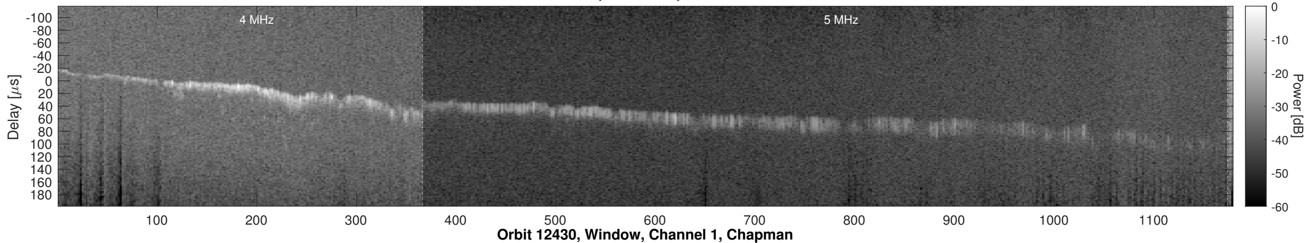
Orbit 12430, Channel 1, Uncorrected
