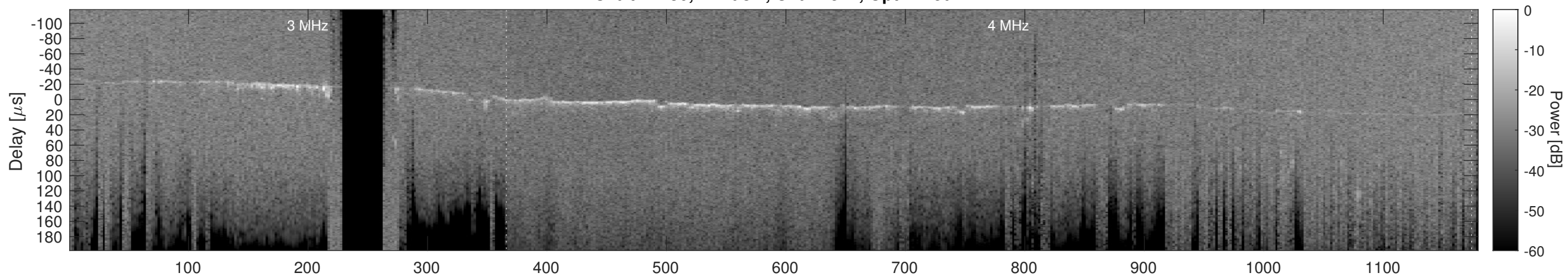
Orbit 12430, Cluttergram
