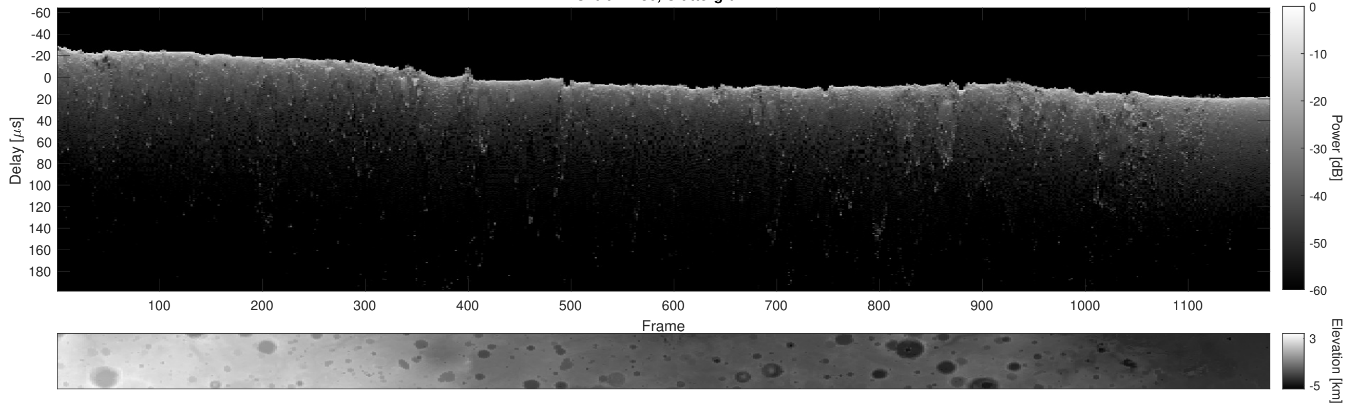
Orbit 12430, Cluttergram
