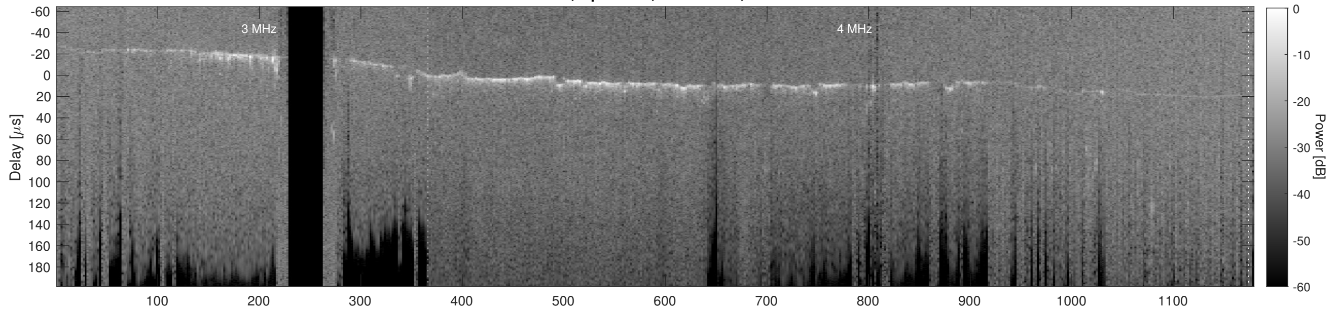
Orbit 12430, Cluttergram
