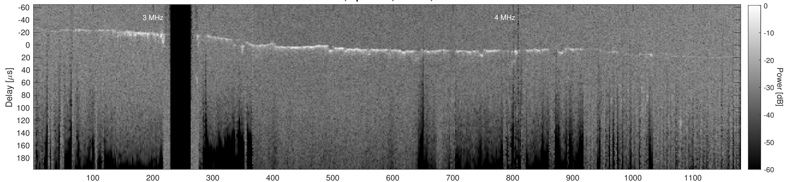
Orbit 12430, Cluttergram
