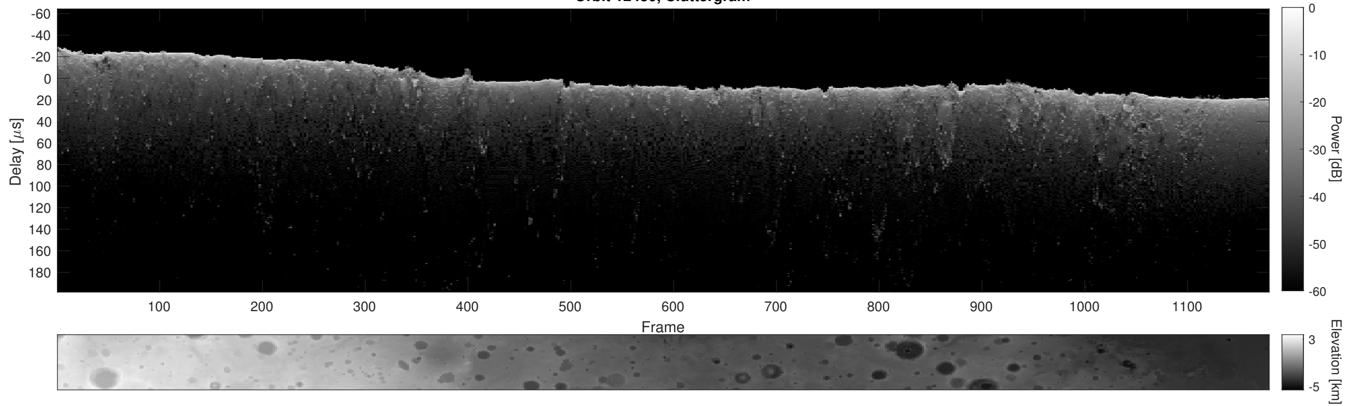
Orbit 12430, Cluttergram
