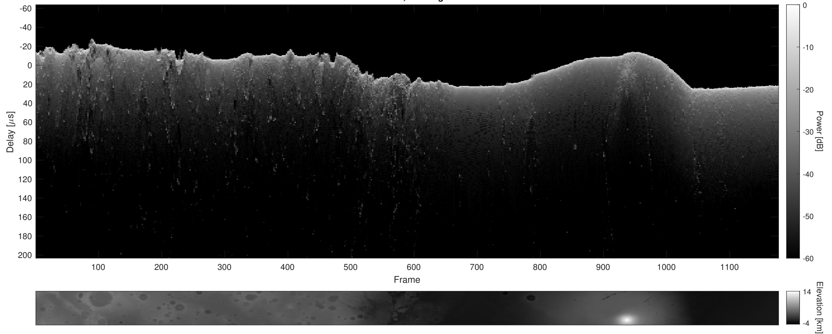
Orbit 12432, Cluttergram
