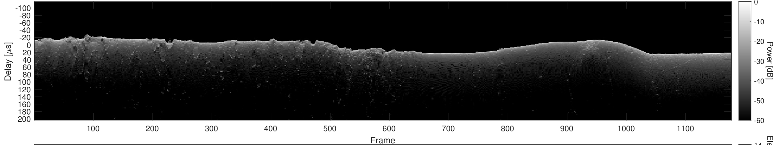
Orbit 12432, Cluttergram
