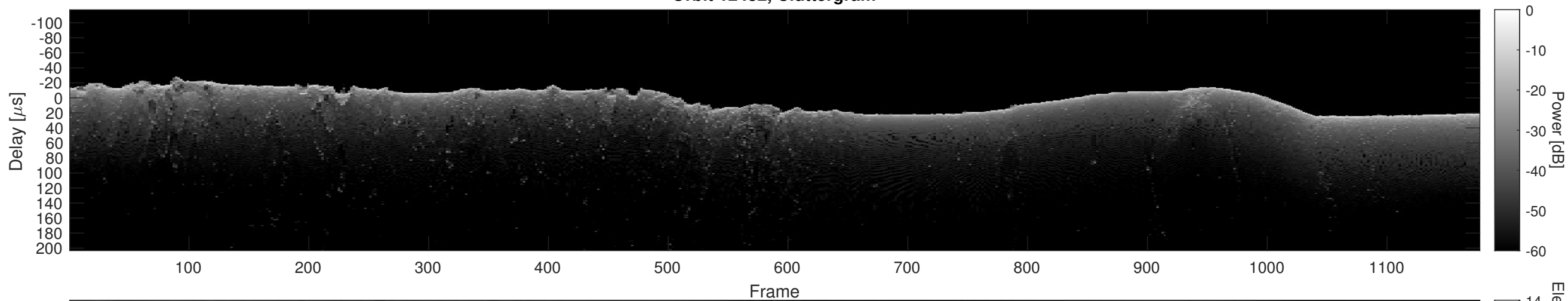
Orbit 12432, Cluttergram
