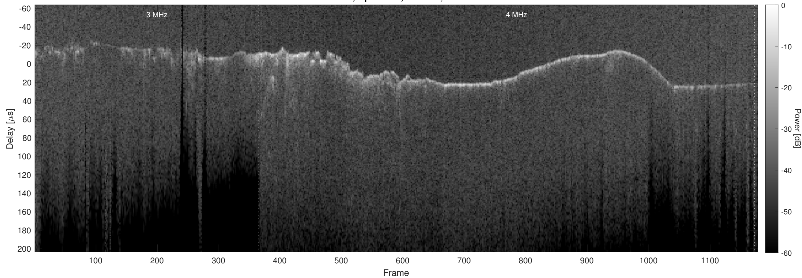
Orbit 12432, Optimized, Window, Channel 2
