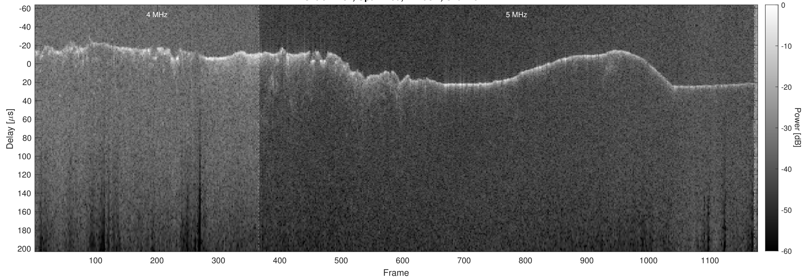
Orbit 12432, Optimized, Window, Channel 2
