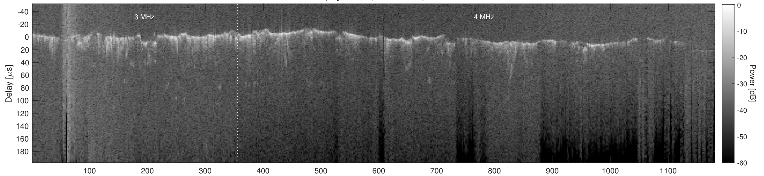
Orbit 12433, Cluttergram
