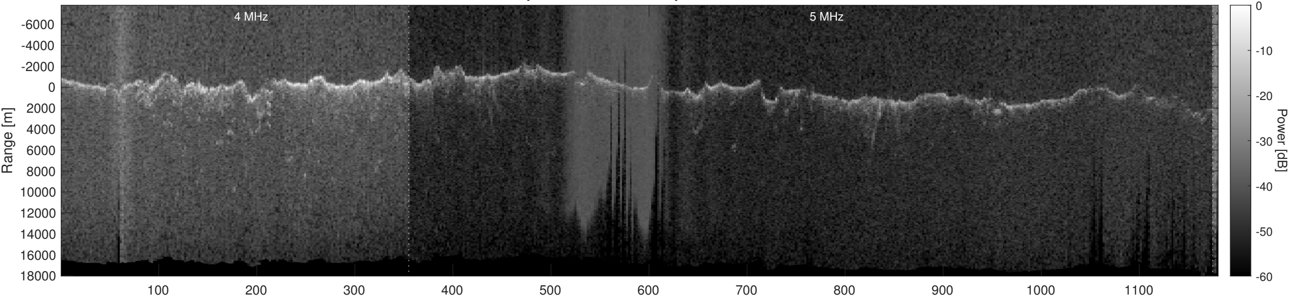
Orbit 12433, Optimized, Window, Depth-Corrected, Channel 2
