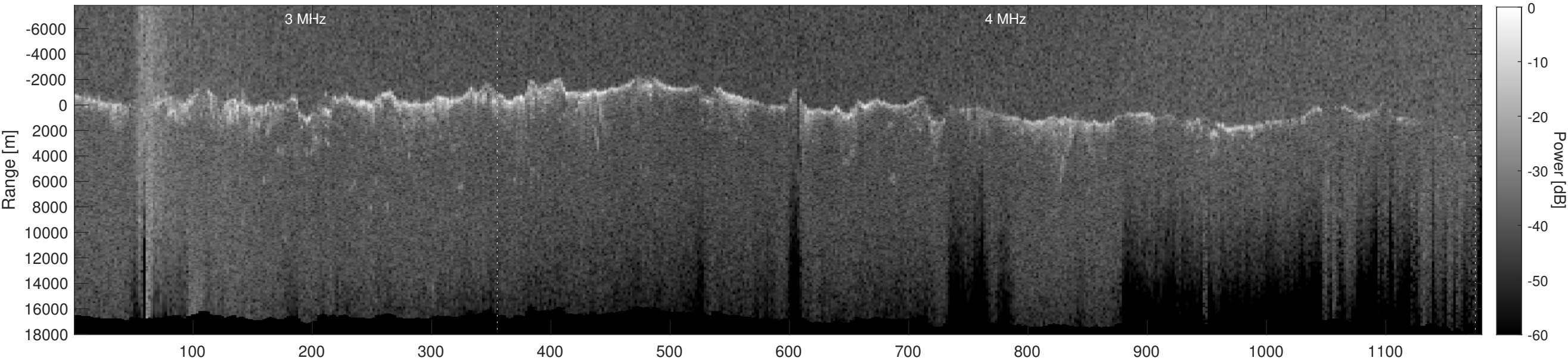
Orbit 12433, Depth-Corrected Cluttergram
