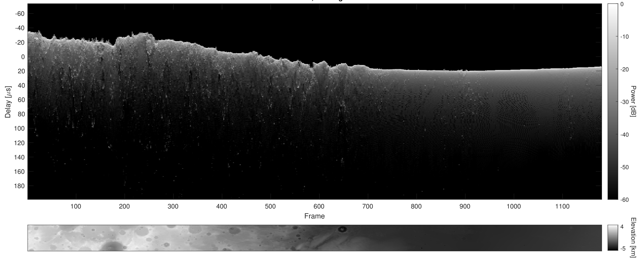
Orbit 12435, Cluttergram
