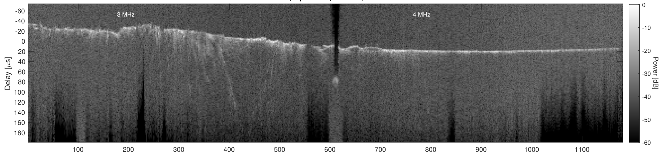
Orbit 12435, Cluttergram
