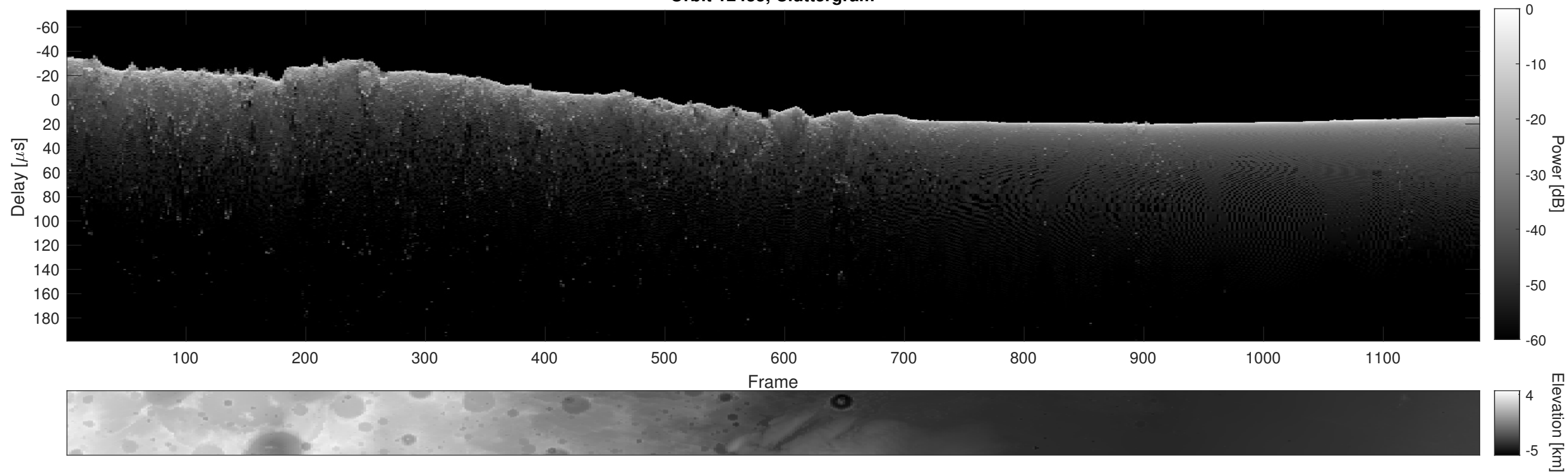
Orbit 12435, Cluttergram
