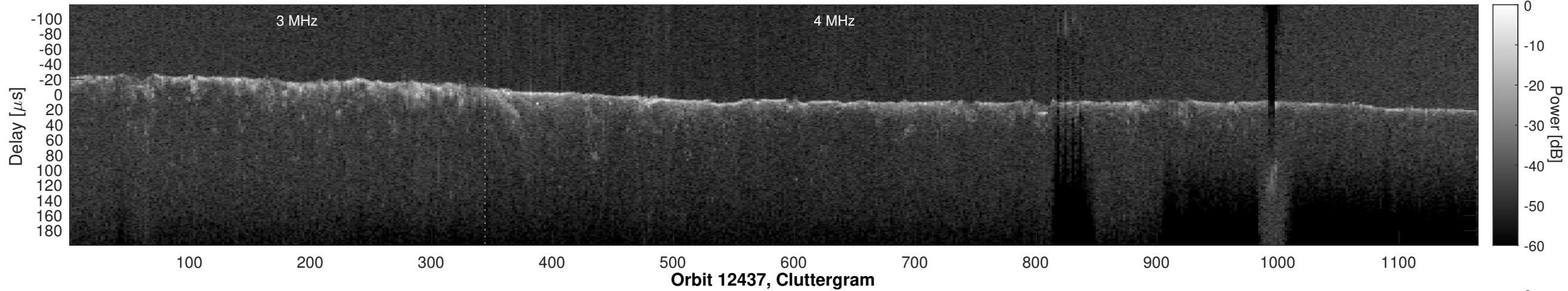
Orbit 12437, Window, Channel 2, Optimized
