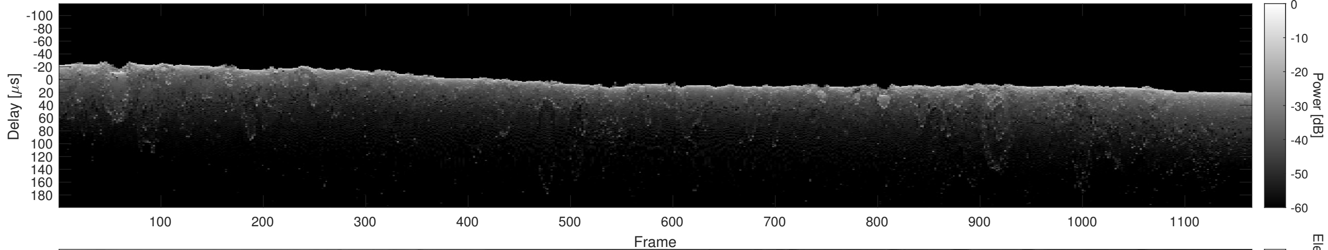
Orbit 12437, Cluttergram
