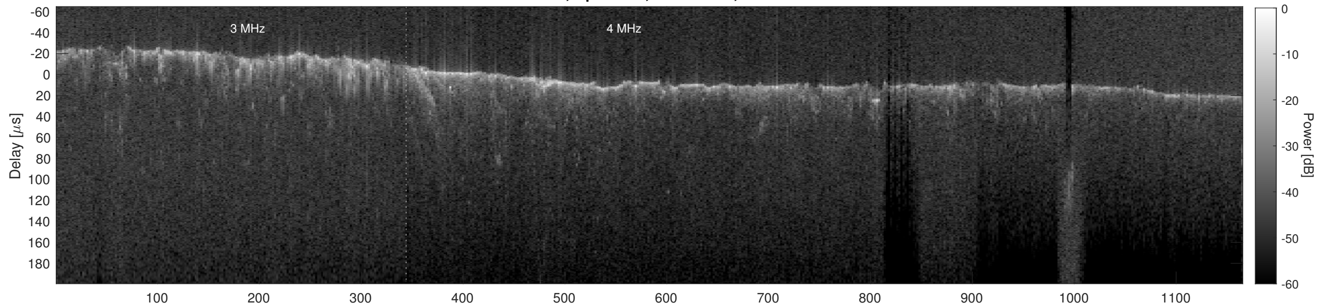
Orbit 12437, Cluttergram
