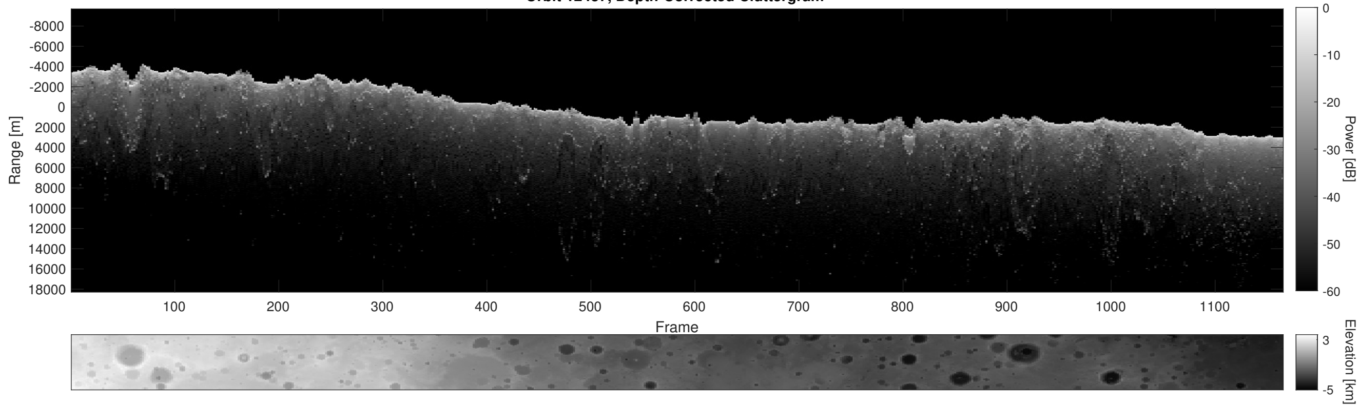
Orbit 12437, Depth-Corrected Cluttergram
