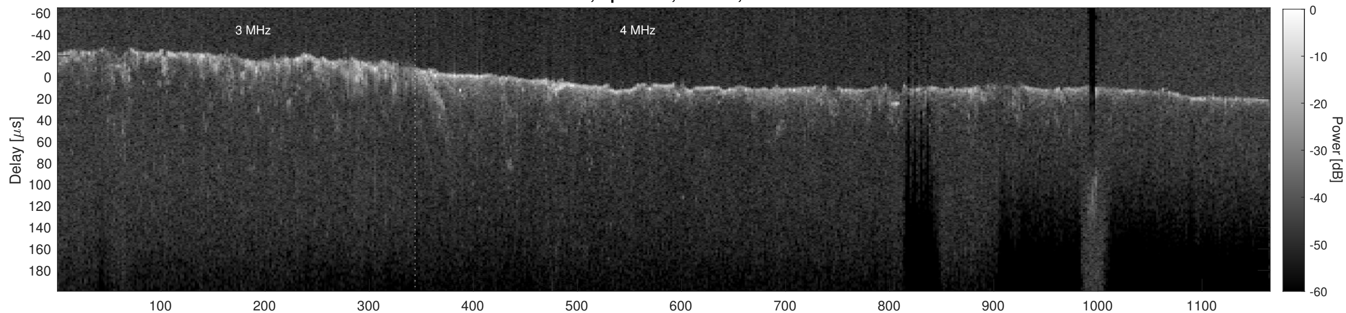
Orbit 12437, Cluttergram
