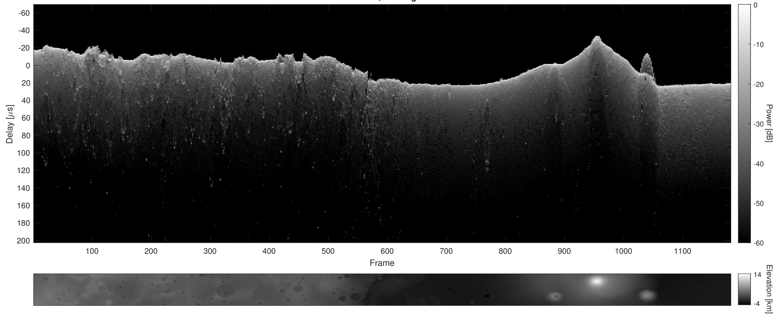
Orbit 12439, Cluttergram
