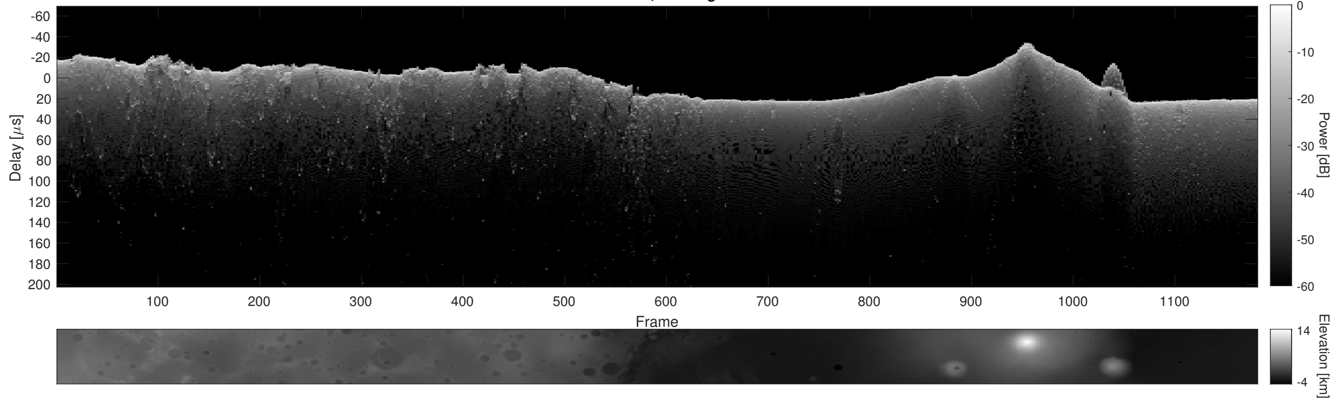
Orbit 12439, Cluttergram
