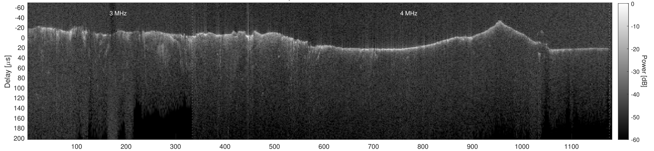
Orbit 12439, Cluttergram
