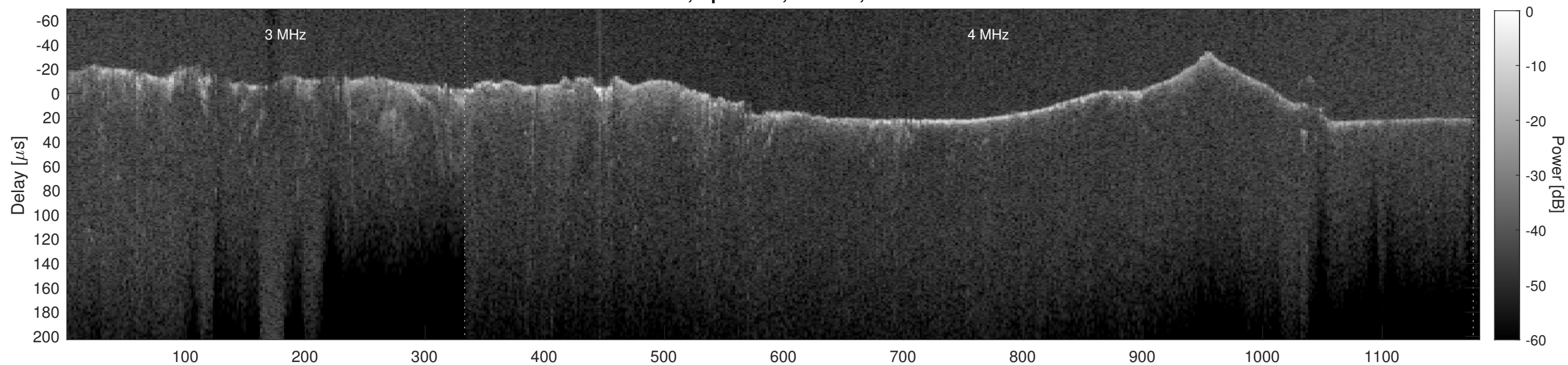
Orbit 12439, Cluttergram
