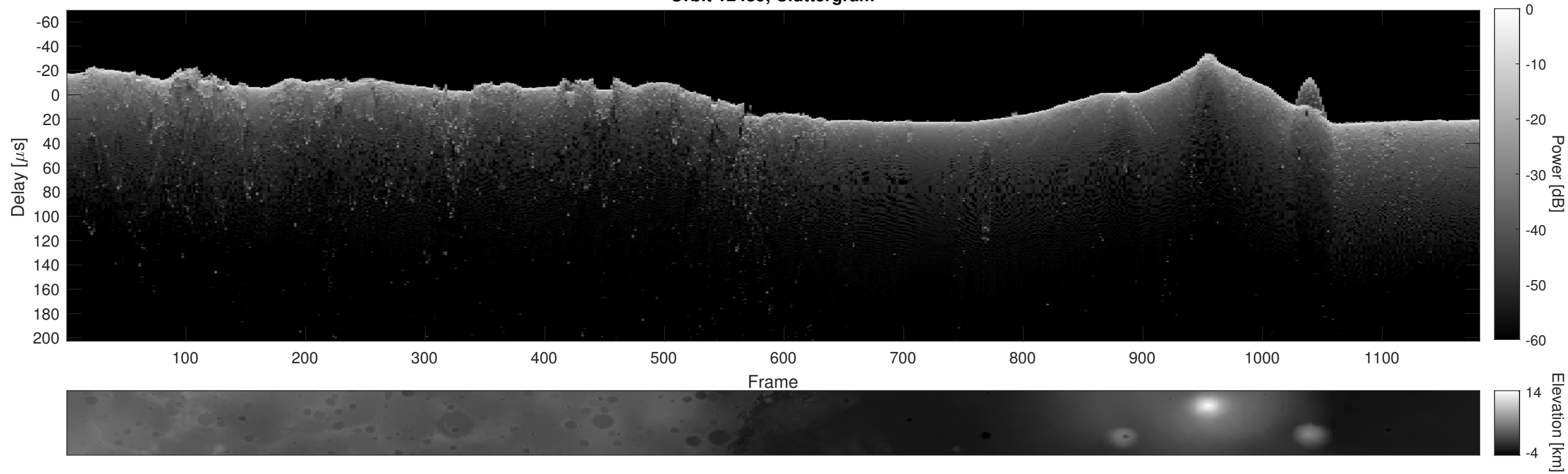
Orbit 12439, Cluttergram
