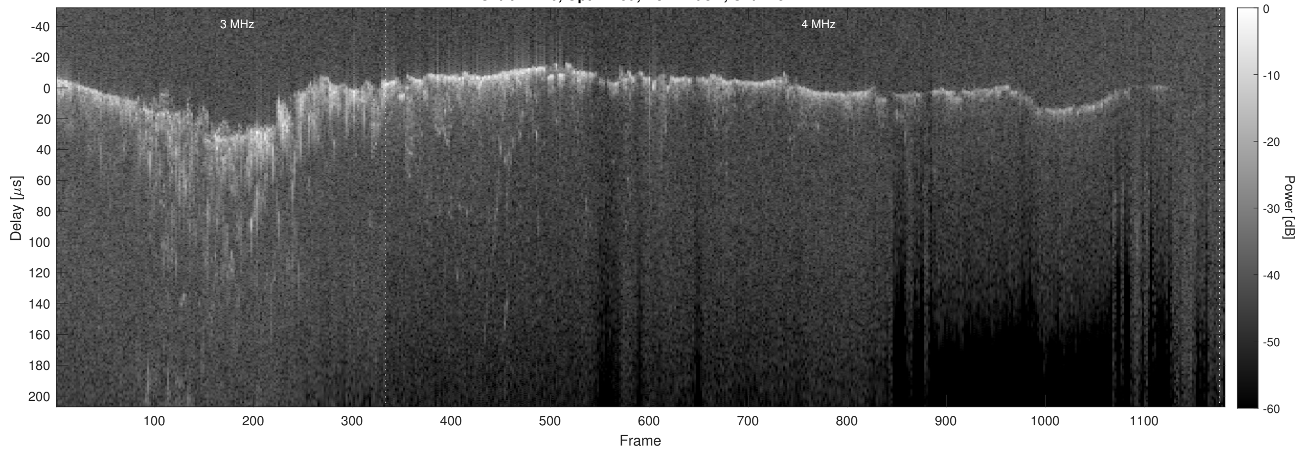
Orbit 12440, Optimized, No Window, Channel 2
