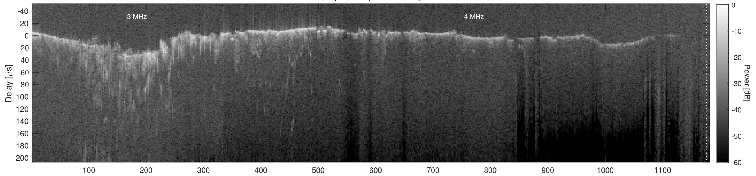
Orbit 12440, Cluttergram
